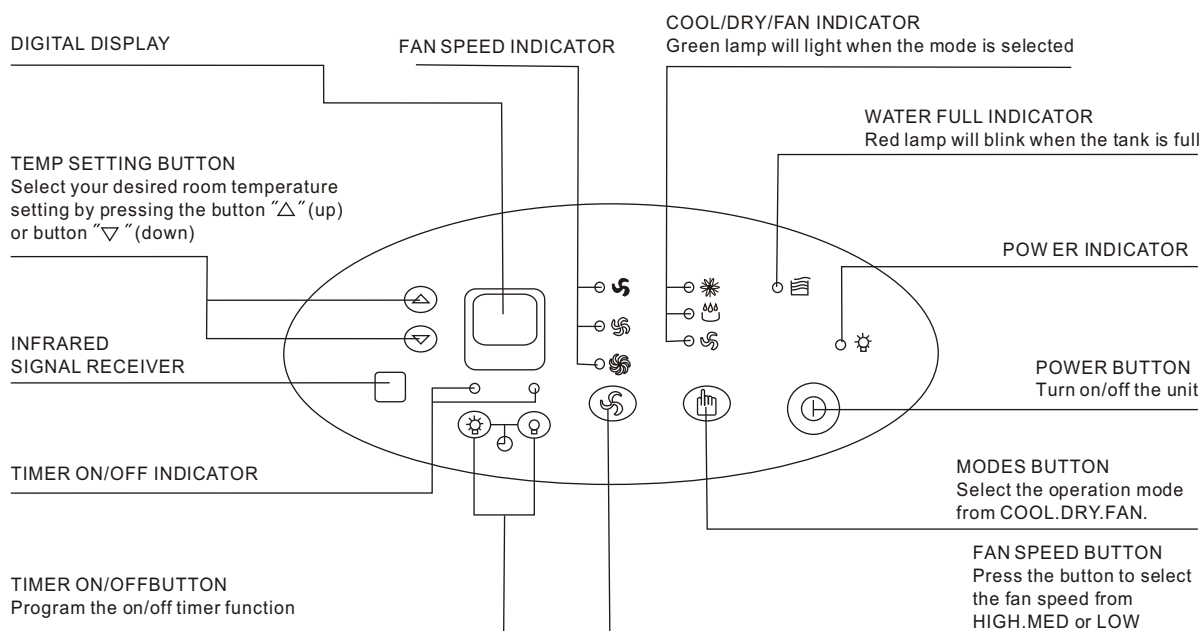
OPERATING PANEL
