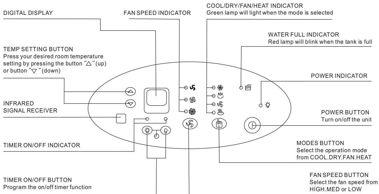
OPERATING PANEL
